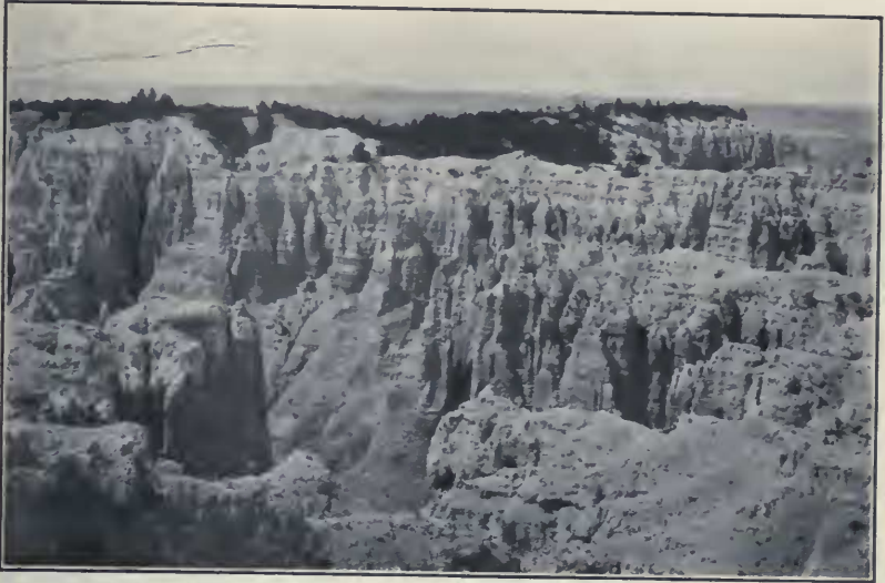
FIG. 1. Section of the Leptauchenia volcanic ash beds in a canyon of Sheep Mountain, Big Badlands. The top of the columnar vertical weathering in the picture is the top of division (a) of the Leptauchenia beds, as described in the text. Above this is the "white ash layer" of Matthew, division (b) of the text. This appears lighter colored than division (a), and does not show vertical columnar weathering.
